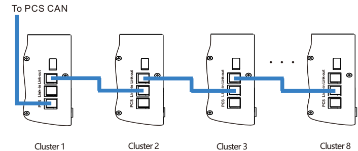
Fig 4.10: Multi-cluster communication wiring
