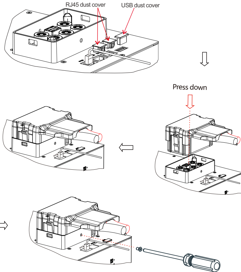
Fig 4.8: Power connection
