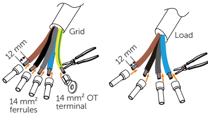
16 Strip 12 mm of L1, L2, L3 and N cables.
