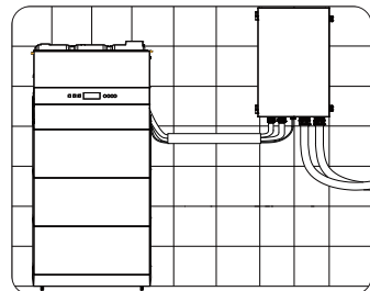
20 Connect the Grid cable to the utility grid and the load cable to the household loads.
