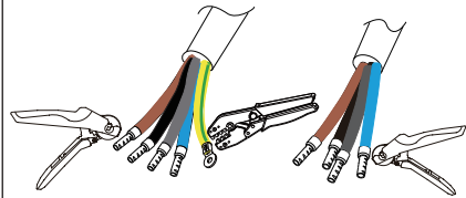
17 Crimp Grid and Load cables.
