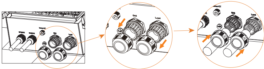
18 Thread Grid and Load cables through the Grid and Load port and then into the meterbox.
