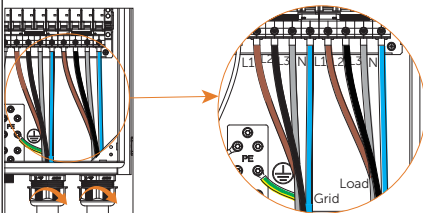
19 Connect Grid and Load cables to the corresponding terminals in the meterbox.
