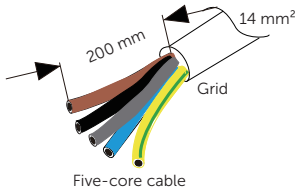
15 Strip Grid and Load cables.
